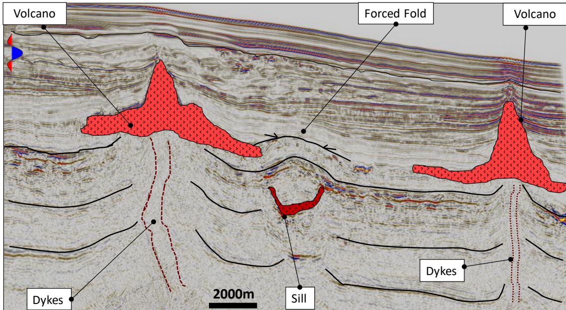
Figure 2.39. Vertical slice showing in-context interpretation suggesting the mound-like features are Volcanoes. Seismic data courtesy of NZP&M.
