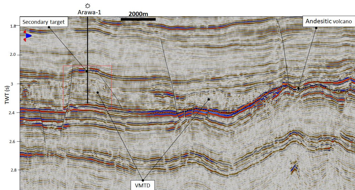
Figure 2.2. Exploration well Arawa-1 drilling into bright spot (andesitic volcanic pile). Notice the andesitic volcano on the right side. Seismic data courtesy of NZP&M. VMT= Volcanic Mass Transport Deposit.
