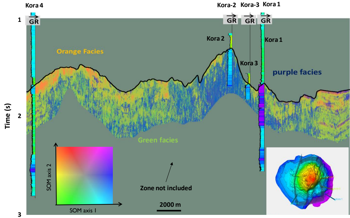
Figure 3.26. Vertical slice connecting the four Kora wells through the SOM clusters showing the two distinctive colors (purple-ish and yellow-ish) indicating two different facies. The green facies represent clastic sediments. Facies are colored based on the latent space projection. (After Infante-Paez and Marfurt 2017) Seismic data courtesy of NZP&M.
