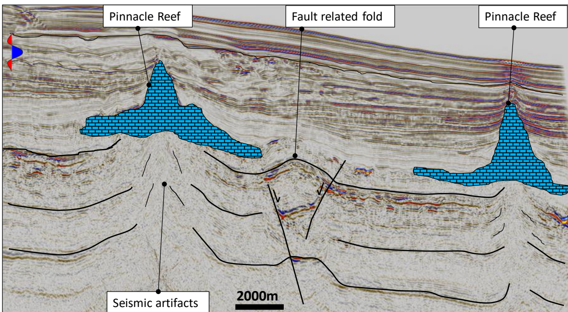
Figure 2.40. Vertical slice showing an incorrect biased interpretation where the mound-like features are carbonate build-ups. Seismic data courtesy of NZP&M.
