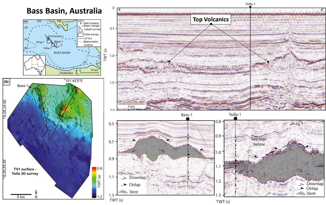
Figure 2.4. Vertical amplitude sections showing exploration wells drilling into mound-like features. The wells drilled a basaltic volcano rather than a carbonate buildup. Map on bottom left is the top of the volcanic units. Notice the dome-like shape. (After Reynolds et al., 2017).
