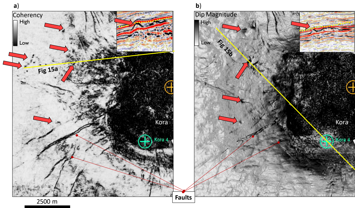
Figure 2.35. (a) Coherence and (b) Horizon slices thought dip magnitude attribute volumes close to the top of the Kora volcano. Reddish arrows point to small circular features in both attributes that represent the small cones. Yellow dotted line in the insert figure represents a reflector close to the base of Kora. Radial low coherence anomalies are normal faults. Kora 3D seismic survey courtesy of NZP&M.
