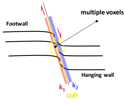
Figure 3.14. Cartoon showing a normal fault and its attribute response. Such red-yellow and blue pattern is easily recognized by a human interpreter. However, since they occur at laterally shifted voxels, they are more difficult to interpret for a machine. Most positive curvature, k_1 (in red) illuminates the footwall, most negative curvature, k_2 (in blue) illuminates the hanging wall, while coherence (in yellow) illuminates the fault discontinuity. After Qi, 2018.
