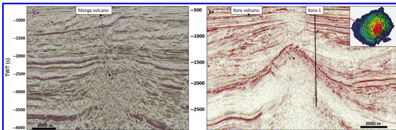
Figure 9. Signal-to-noise comparison between (a) legacy 2D ES-89 seismic survey from 1989 and (b) modern 3D Kora 3D 2006 seismic survey. Notice the higher quality image of the Kora Volcano compared with the Manga Volcano. Seismic data courtesy of NZP&M.
