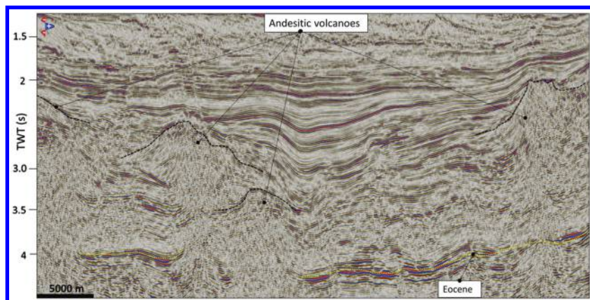
Figure 10. Seismic section from P95 2D seismic survey showing several undrilled mound-like structures interpreted as andesitic volcanoes. Seismic data courtesy of NZP&M.
