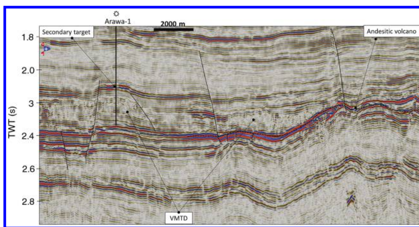
Figure 2. Exploration well Arawa-1 drilling into a bright spot (andesitic volcanic pile). Notice the andesitic volcano on the right side. VMT, volcanic mass transport deposit. Seismic data courtesy of New Zealand Petroleum and Minerals (NZP&M).
