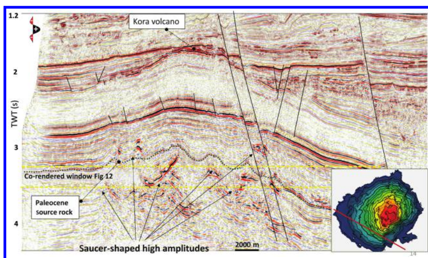
Figure 13. Vertical seismic section from the Kora 3D seismic survey showing interpreted saucer-shaped sills intruding into the Paleocene Waipawa marine source rock and possibly creating an atypical petroleum system, such as the one proposed by Del Pino and Bermudez (2009). After Infante-Paez and Marfurt (2017). Seismic data courtesy of NZP&M.
