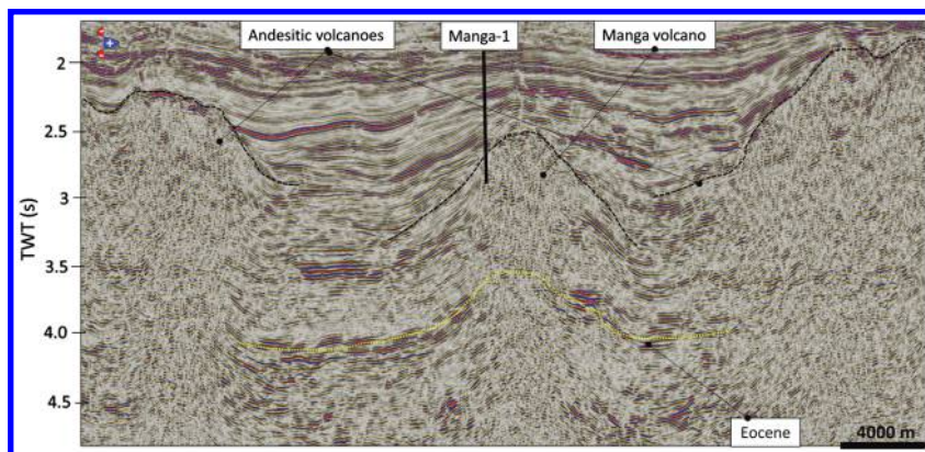
Figure 7. Vertical seismic section from P95 2D seismic survey showing well Manga-1 drilling an andesitic volcano, the Manga Volcano. Seismic data courtesy of NZP&M.
