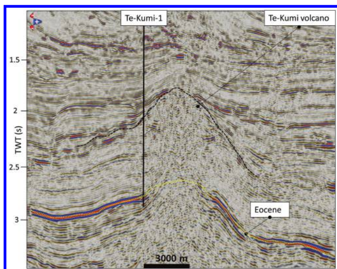
Figure 8. Vertical seismic section from P95 2D Survey showing well Te Kumi-1 drilling an andesitic volcano, Te-Kumi Volcano. Seismic data courtesy of NZP&M.
