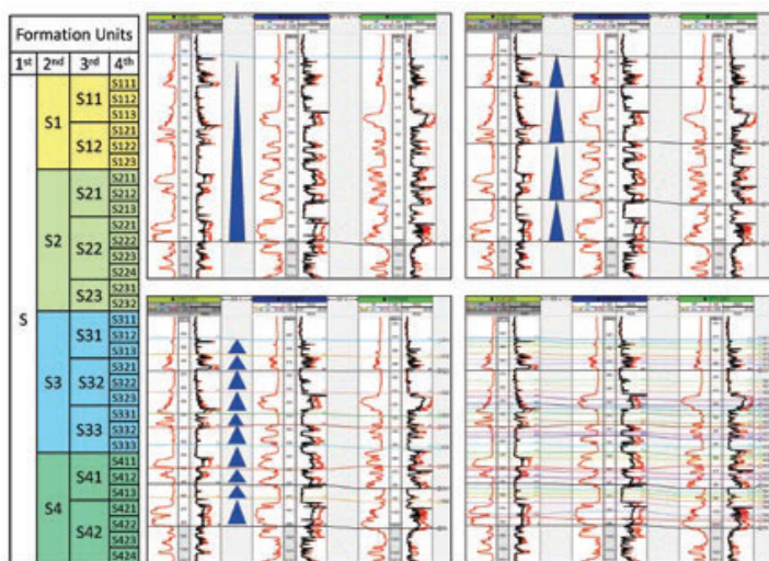
Figure 1. Three representative well logs showing the first, second, third, and fourth-order sequences.
